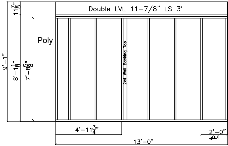
Shear Wall A
