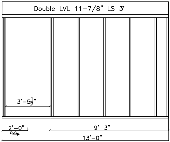
Shear Wall B
