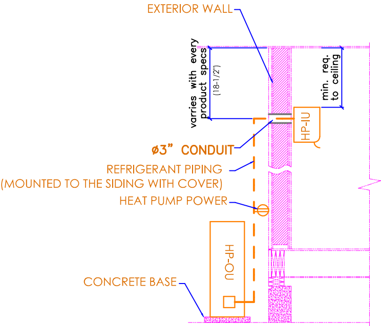
SECTION "Y" STANDARD HEAT PUMP INSTALL
